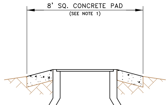
TOP OF MANHOLE IN UNIMPROVED AREA
